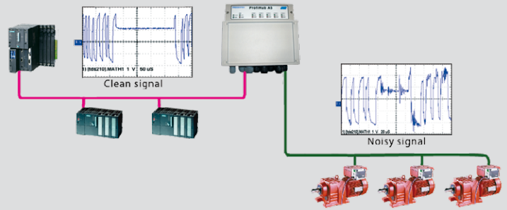
Example of the barrier function of the ProfiHub. Noise and EMC disturbances will not affect the backbone or the other channels
