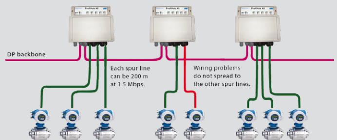
Example of dynamic spur lines to instruments. The devices can be added and removed during operation.
